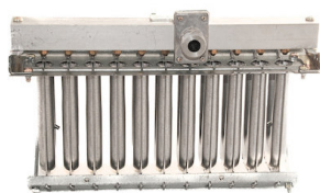
Main Burner & Bar (Nut Connection) Morco Primo MP11 (MP0082)
