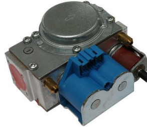
24i RSF Gas Valve (87161424300)
