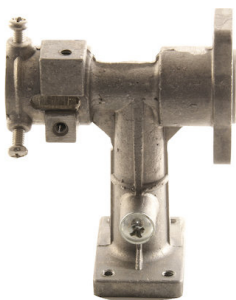
Gas Valve / Burner Manifold (Direct Connection) MP6 & MP11 (MP0260)
