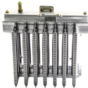
Main Burner & Bar (Nut Connection) Morco Primo MP6 (MP0081)
